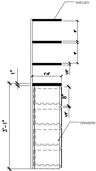
SECTION VIEW (A)
